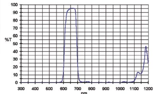
Spectral trace BAADER UV/IR-Cut Filter & BAADER RG 610 Red Color Filter, working as H- \alpha pass-filter
